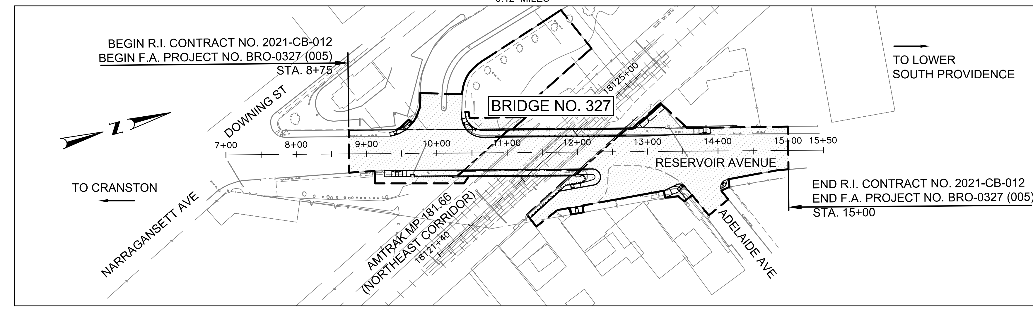
LAYOUT PLAN SCALE: 1" = 80'
