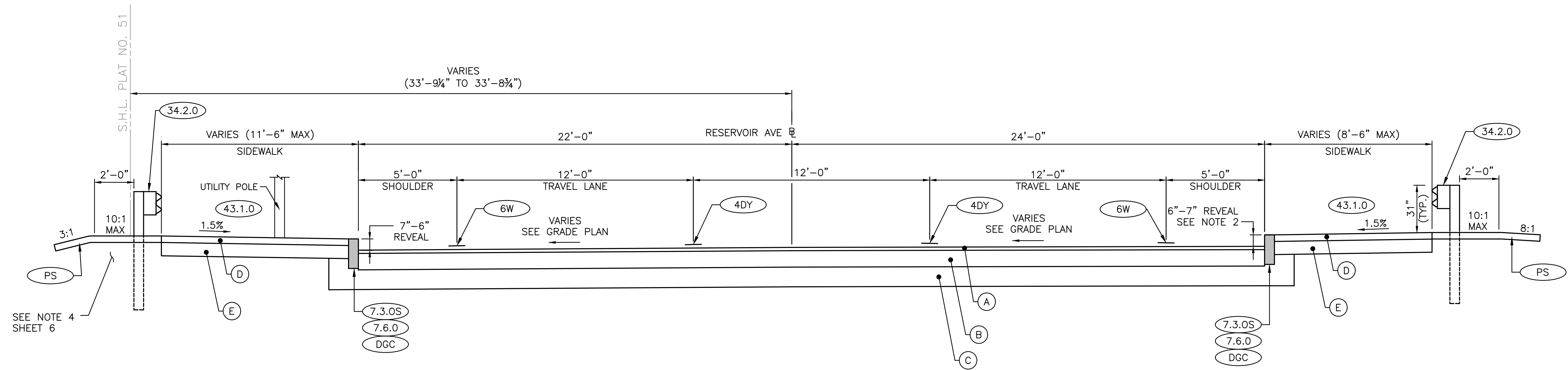
PROPOSED TYPICAL SOUTH BRIDGE APPROACH SECTION STA. 10+25 TO 10+70 SCALE: NTS
