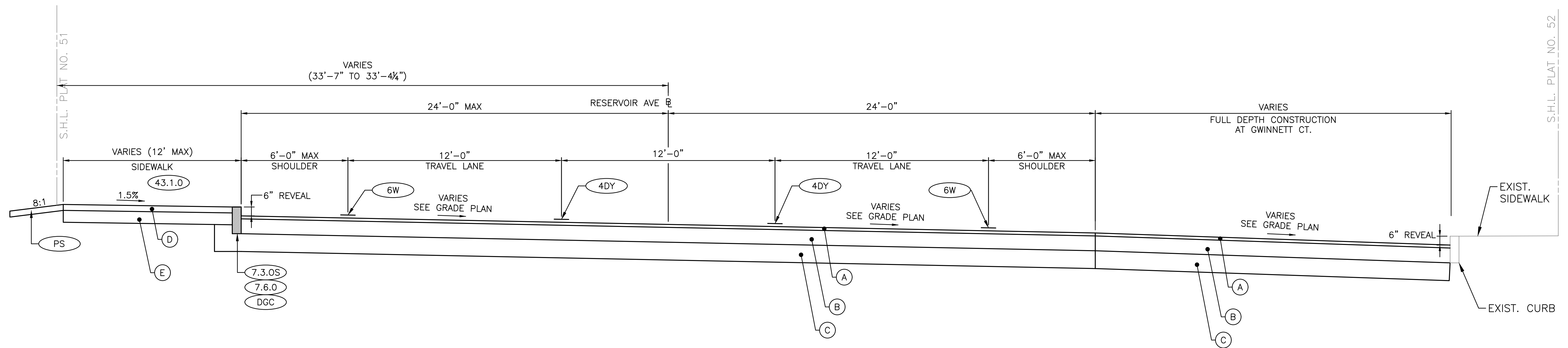
PROPOSED TYPICAL NORTH APPROACH SECTION STA. 12+30 TO 14+75 SCALE: NTS
