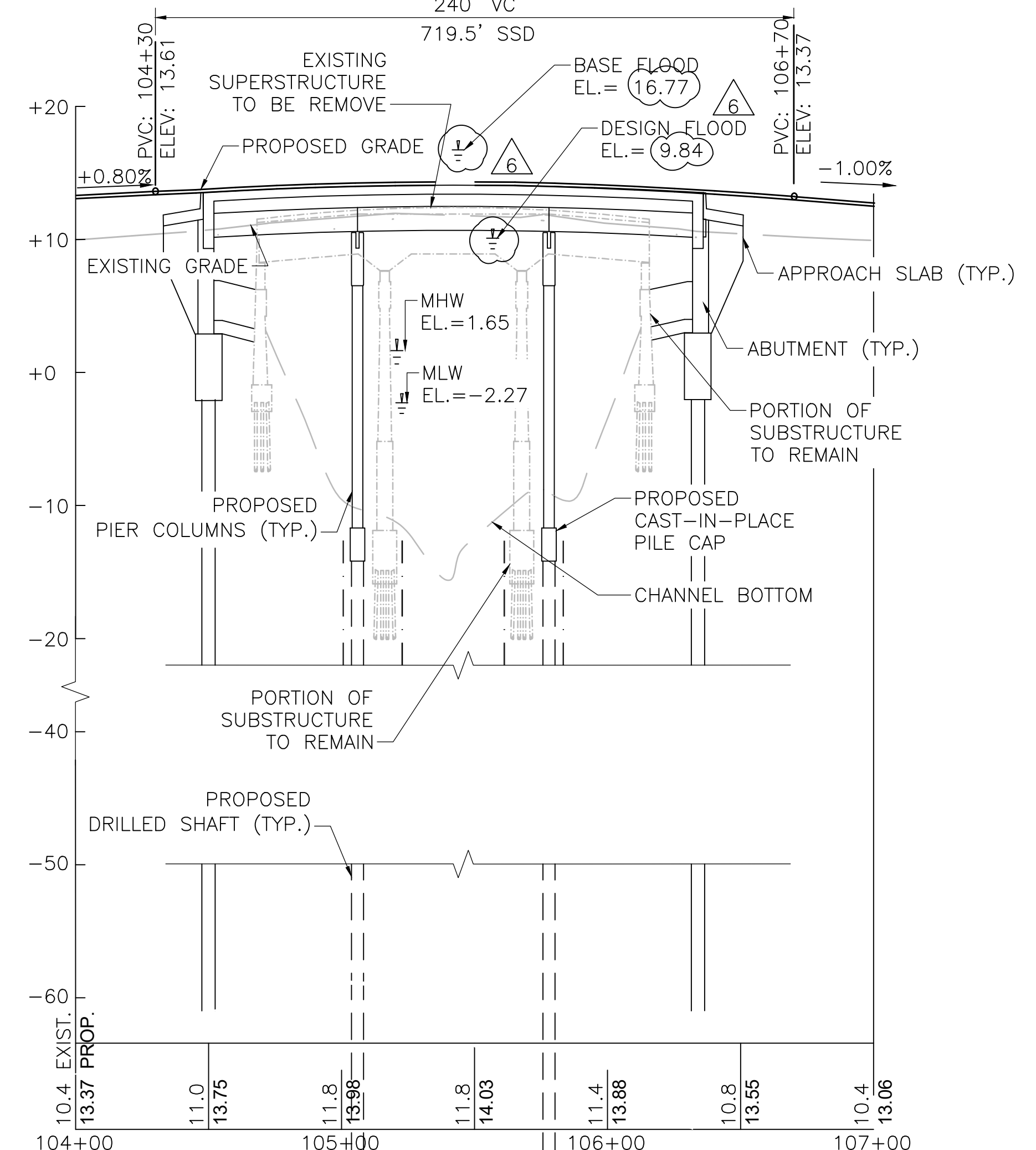
PROFILE ALONG MARION ROAD (US 6) HORIZONTAL 1" = 40' VERTICAL 1" = 8'
