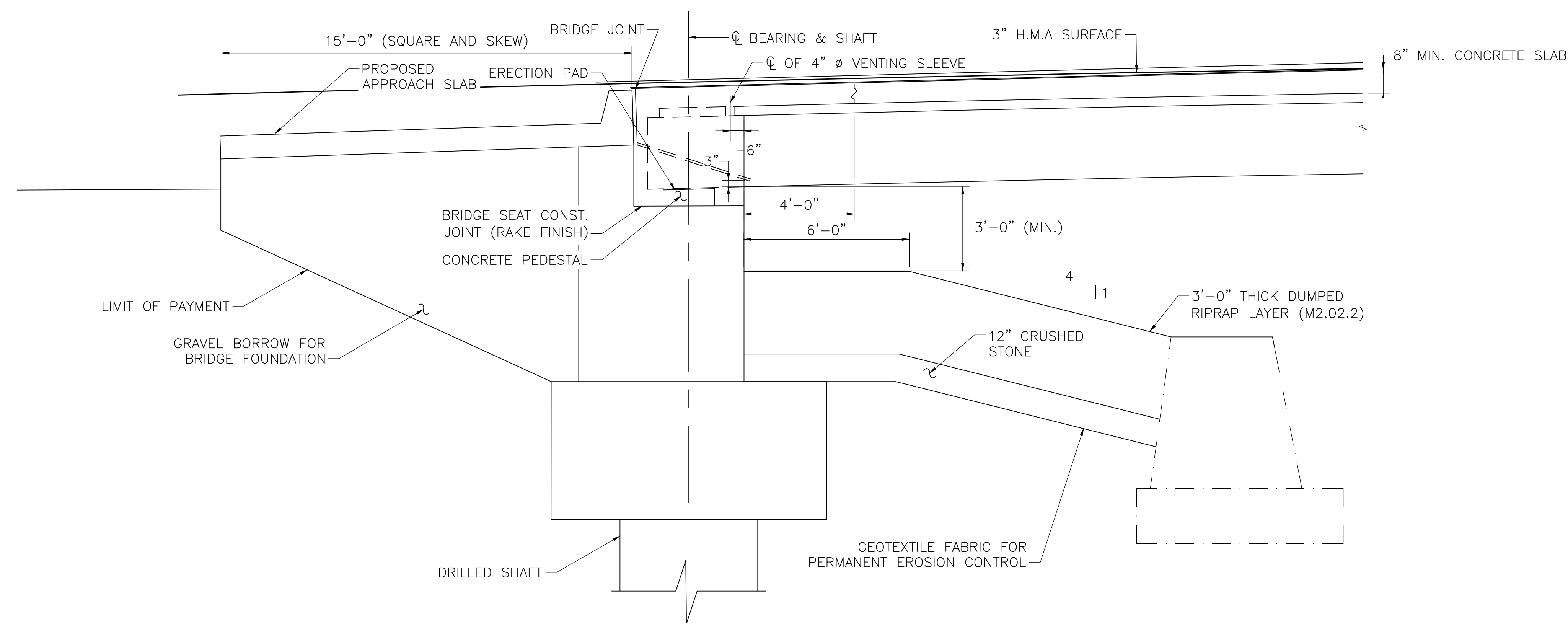
TYPICAL ABUTMENT SECTION WEST ABUTMENT SHOWN (EAST ABUTMENT SIMILAR) SCALE: 3/8" = 1'-0"
