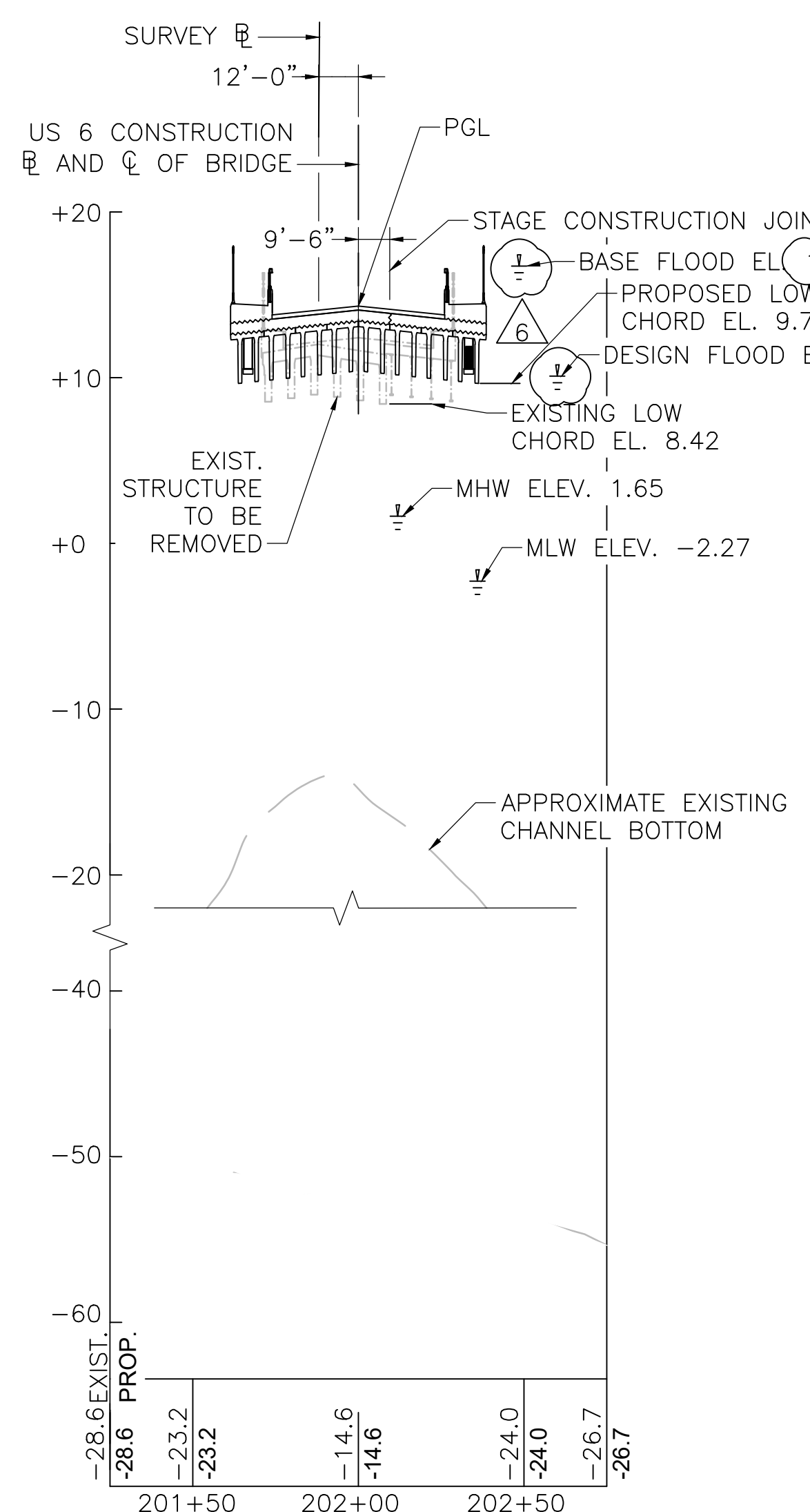
CHANNEL PROFILE (LOOKING UPSTATION) HORIZONTAL 1" = 40' VERTICAL 1" = 8'
