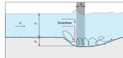
Figure 7.2. Definition sketch for pier scour.
