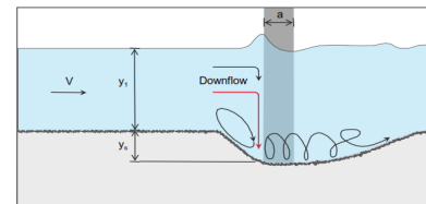
Figure 7.2. Definition sketch for pier scour.
