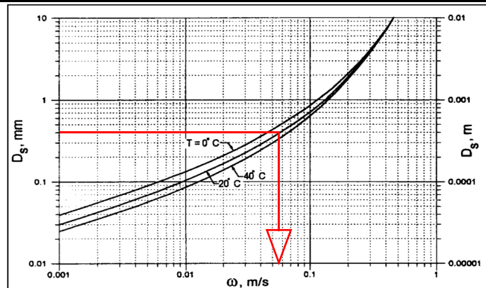
(Figure 6.8, p.6.11, HEC-18)
