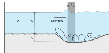
Figure 7.2. Definition sketch for pier scour.
