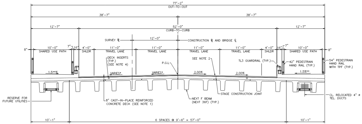
Figure 55. Superstructure Design for Bent 2 and 3 Applied for Hydraulic Analysis
