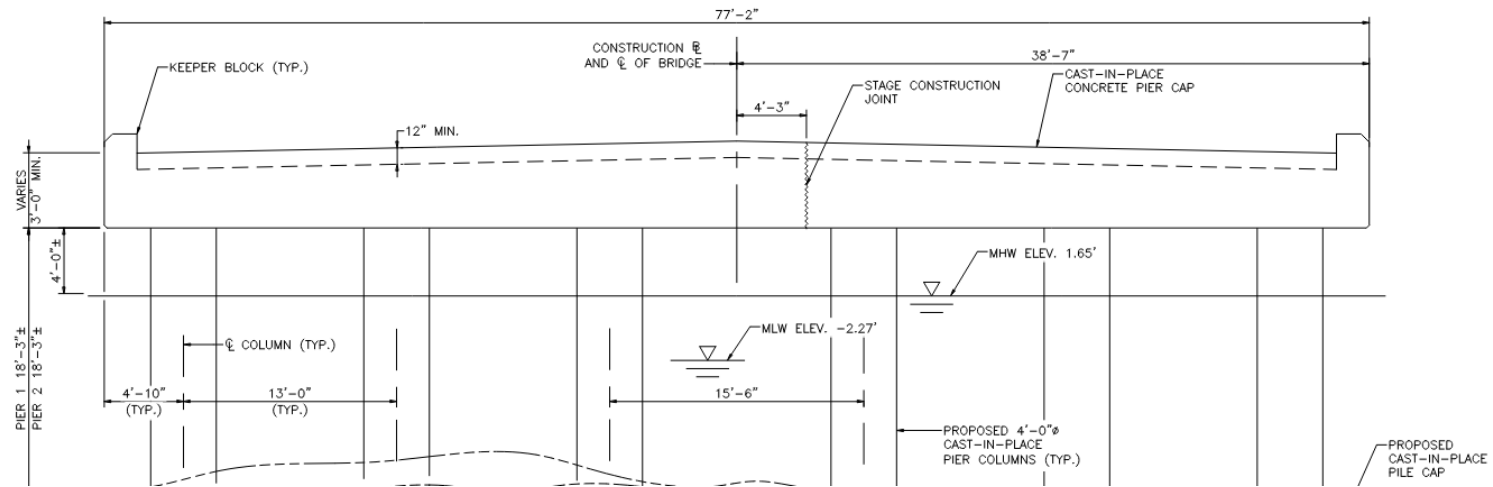
Figure 56. Pile Bent Elevation for Bent 2 and 3
