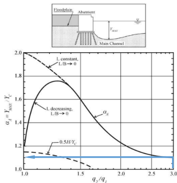
Figure 12-2. Design curve for short-contraction, scour-amplification factor, \alpha_s , for wing-wall abutments subject to Scour Condition A (fixed floodplain)
