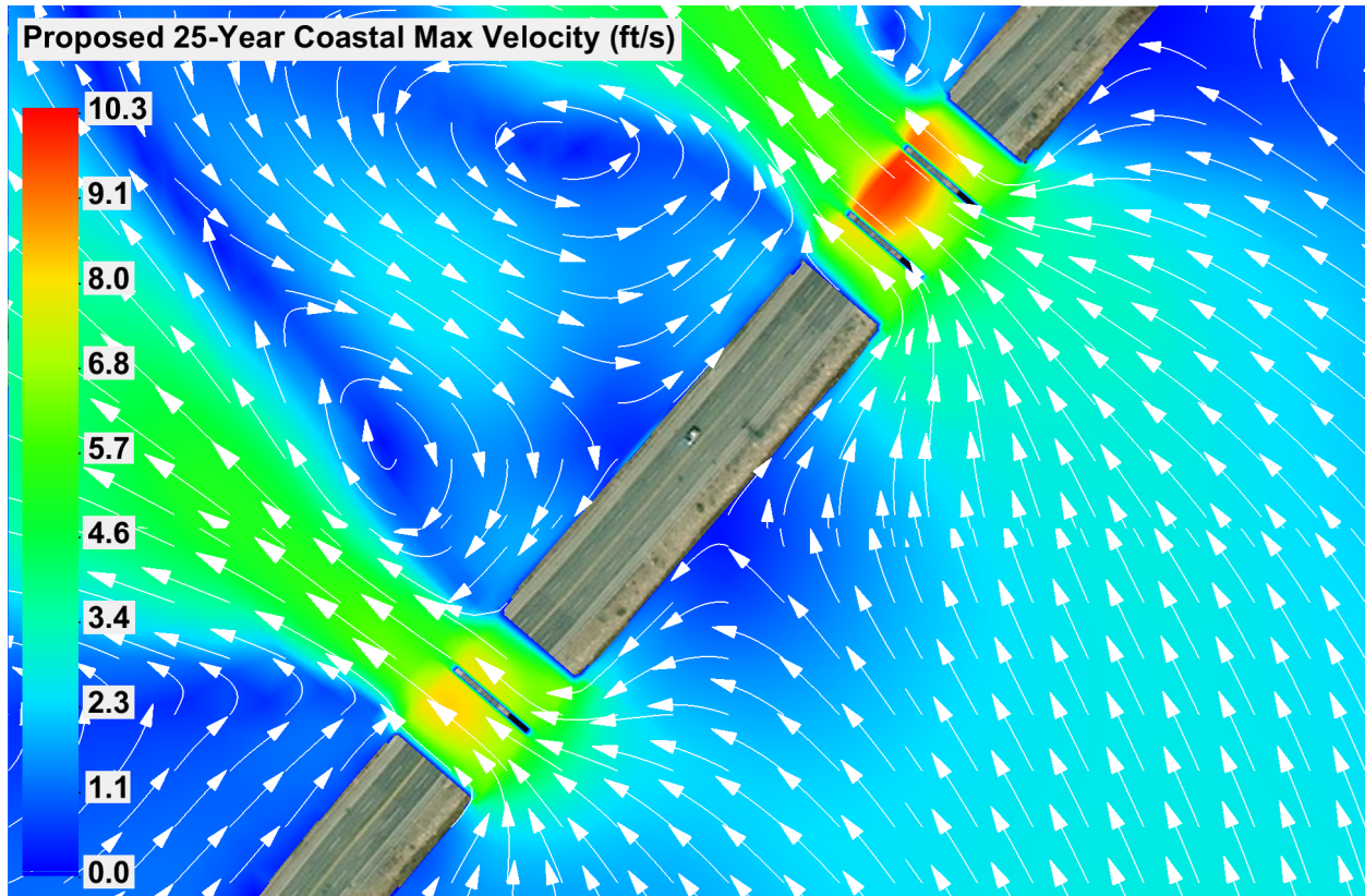
Figure 46. Proposed 25-Year Coastal Max Velocities
