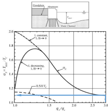
Figure 12-2. Design curve for short-contraction, scour-amplification factor, \alpha_s , for wing-wall abutments subject to Scour Condition A (fixed floodplain)
