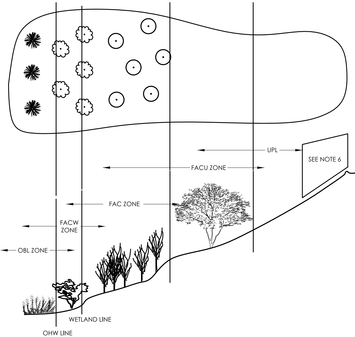
SCHEMATIC PLANTING
