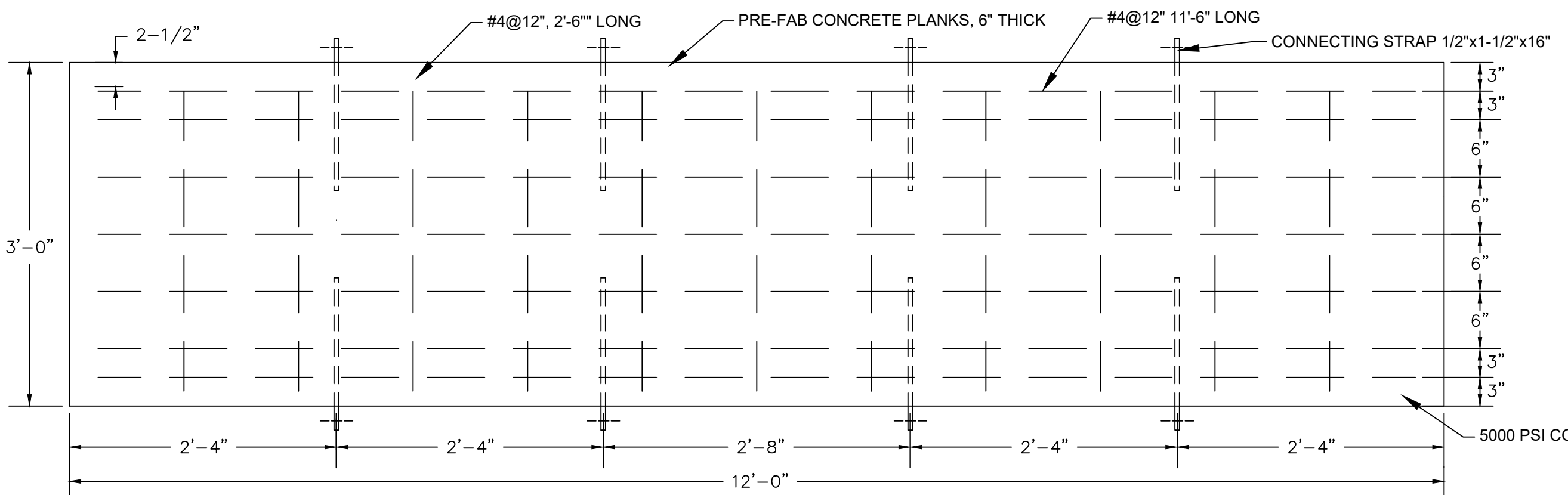
PRE-FAB CONCRETE PLANK PLAN VIEW SCALE: 1"=2'
