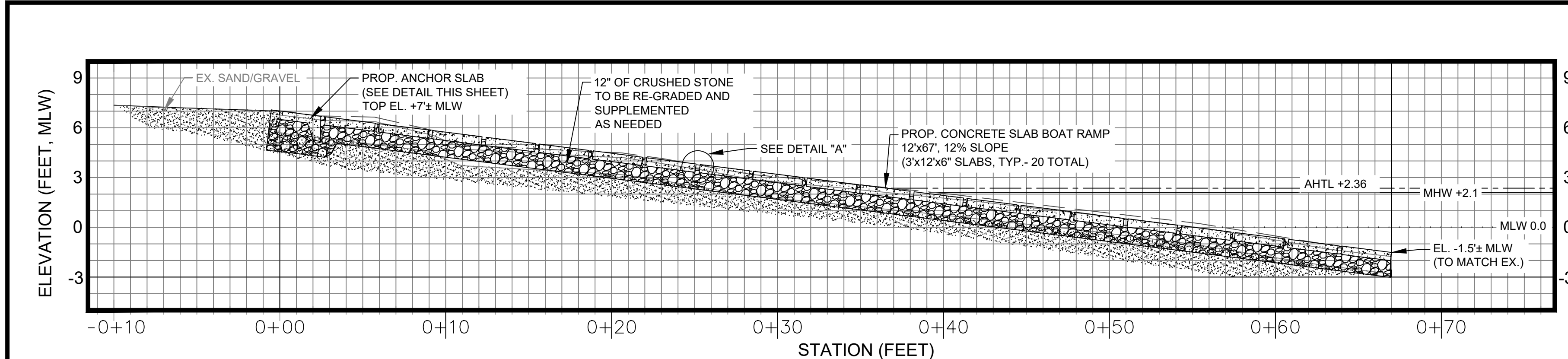
PROPOSED CONDITIONS PROFILE VIEW A-A' SCALE: 1"=5'
