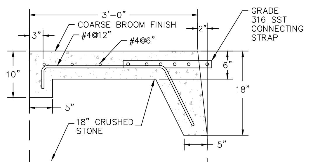
CAST-IN-PLACE ANCHOR SLAB SECTION VIEW SCALE: 1"=1'
