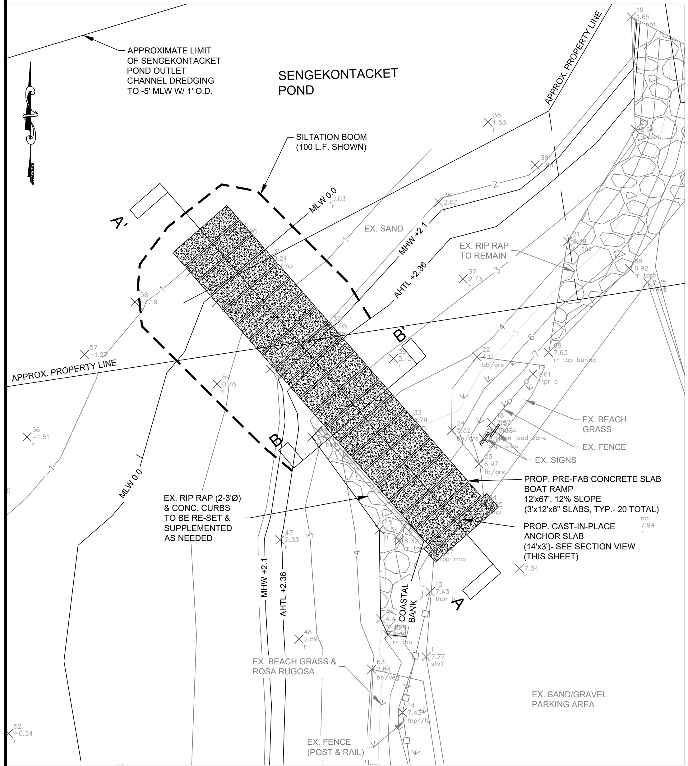
PROPOSED CONDITIONS PLAN VIEW SCALE: 1"=10'
