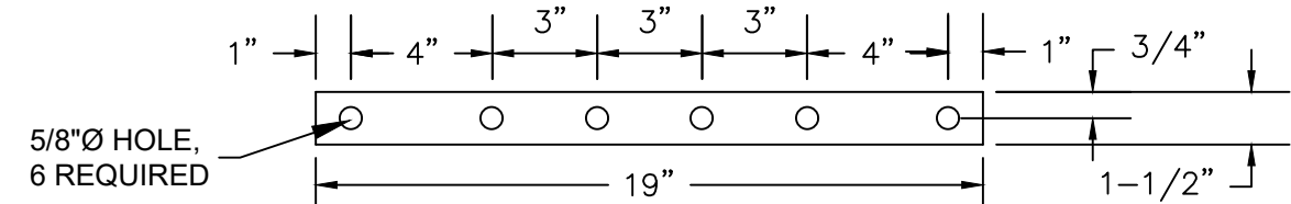
CAST-IN-PLACE ANCHOR SLAB CONNECTING STRAP ELEVATION VIEW SCALE: 1"=1/2'
