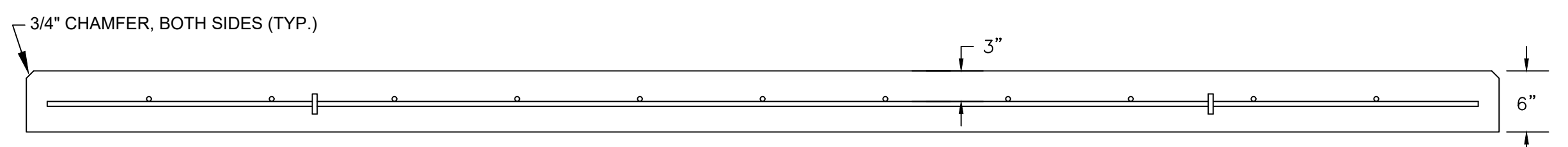
PRE-FAB CONCRETE PLANK ELEVATION VIEW SCALE: 1"=2'
