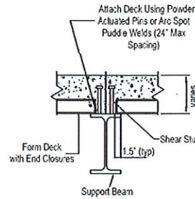
Section View Option #1
