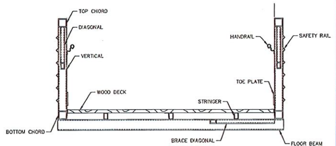
Connector® - Underhung Floor
