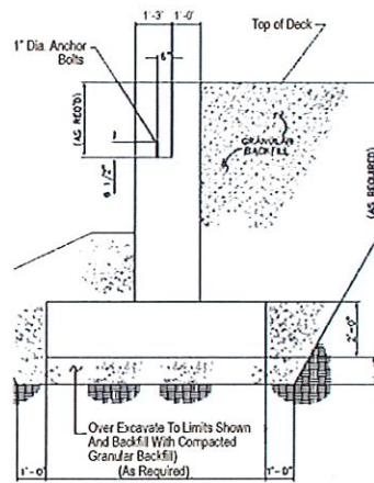
Soil Supported
