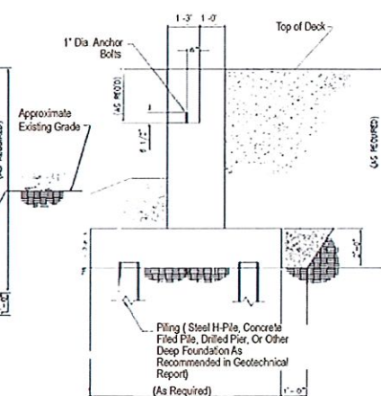
Pile Supported
