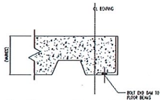
End Dam Detail
