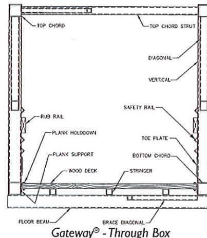
Gateway® - Through Box
