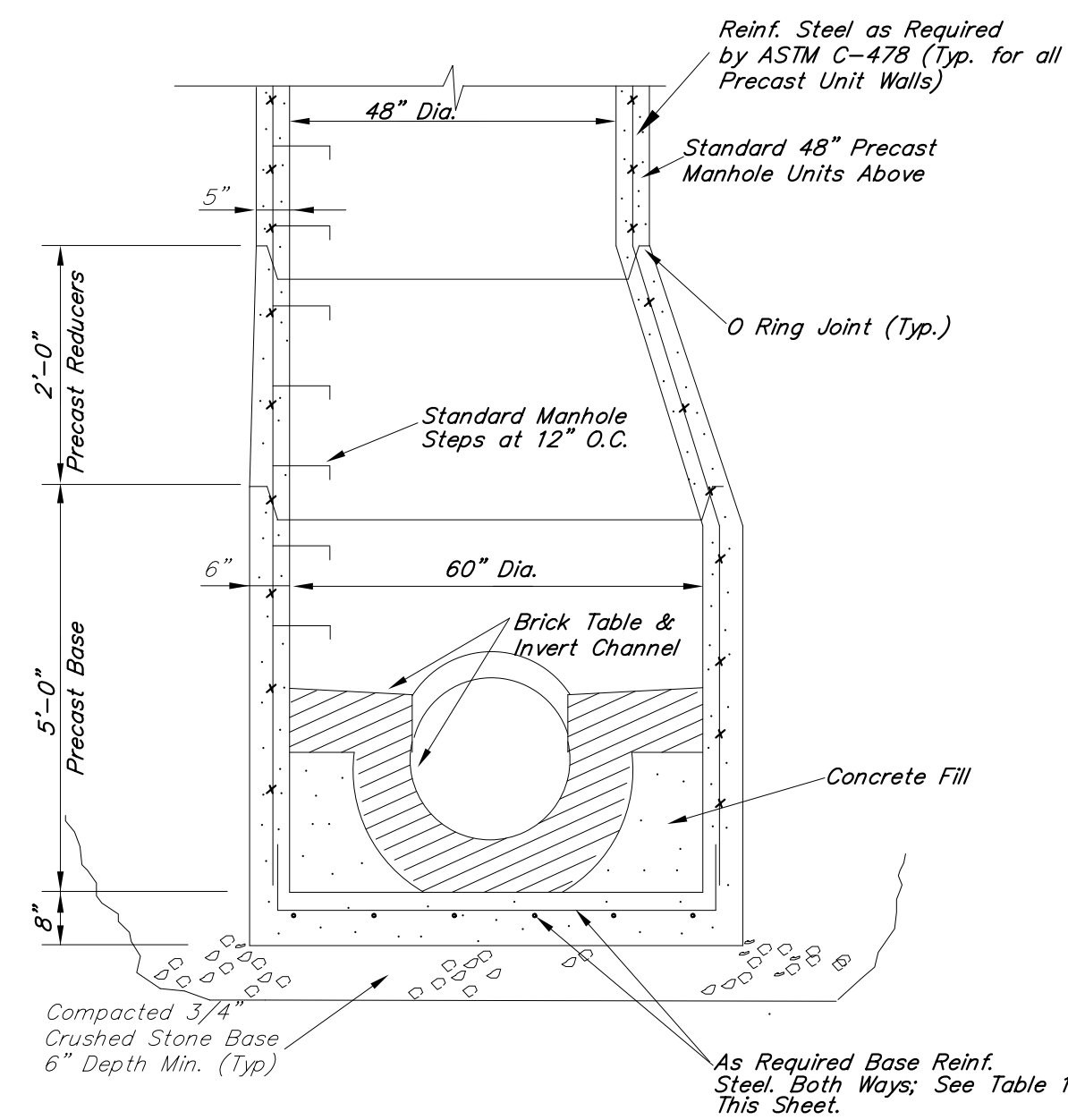
60" I.D. MANHOLE BASE DETAIL
