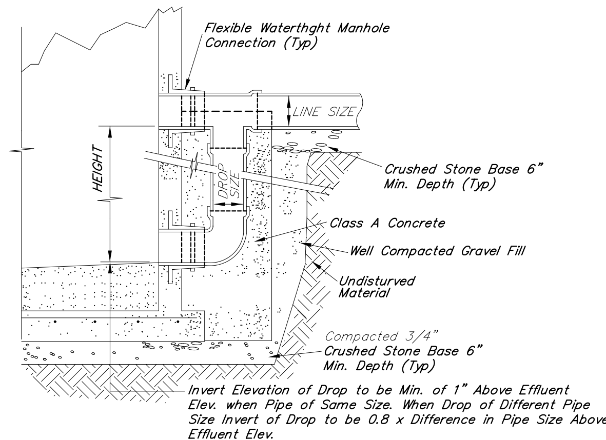
SECTION B-B
