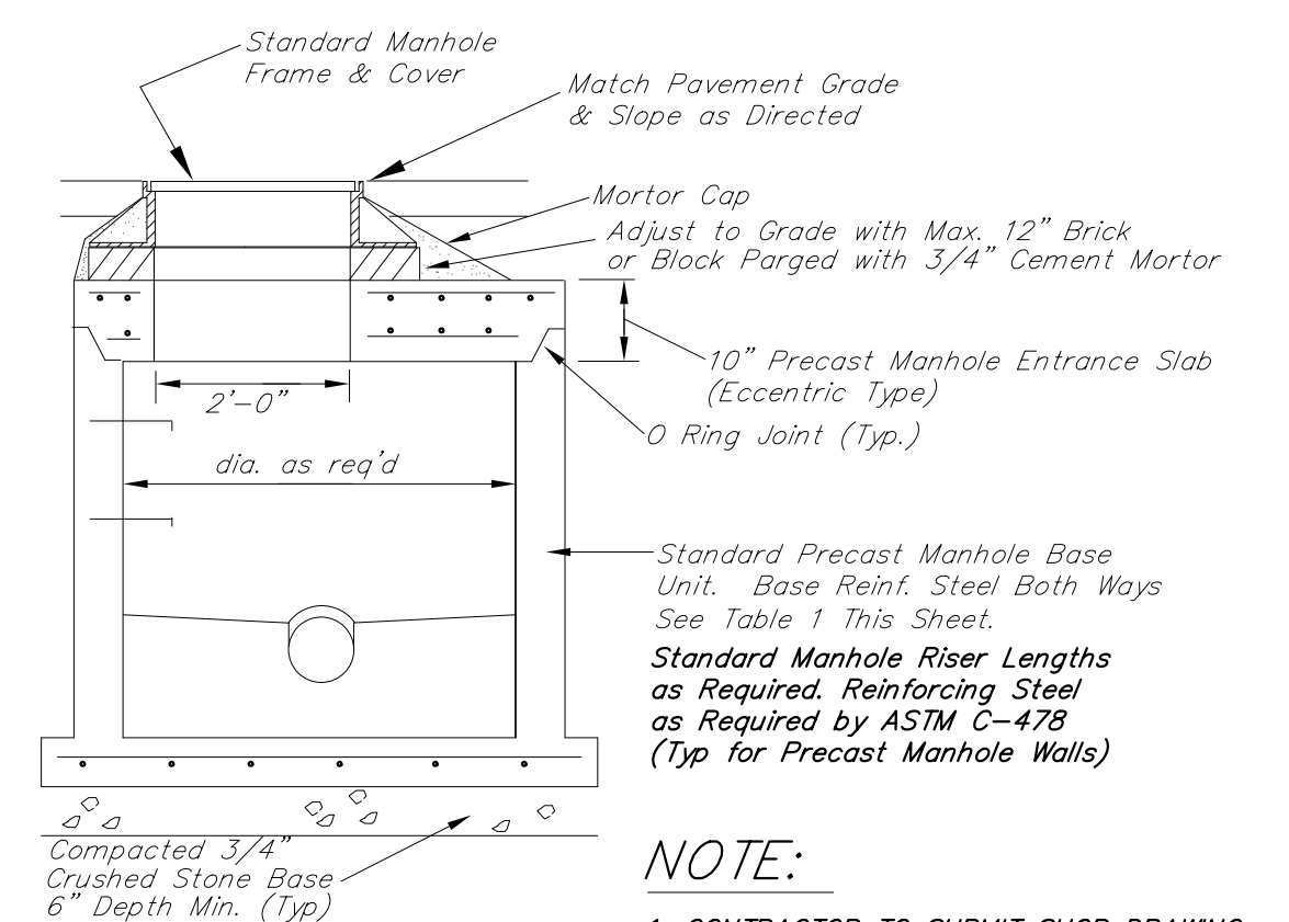
SPECIAL MANHOLE DETAILS Scale: 1/2"=1'-0"
