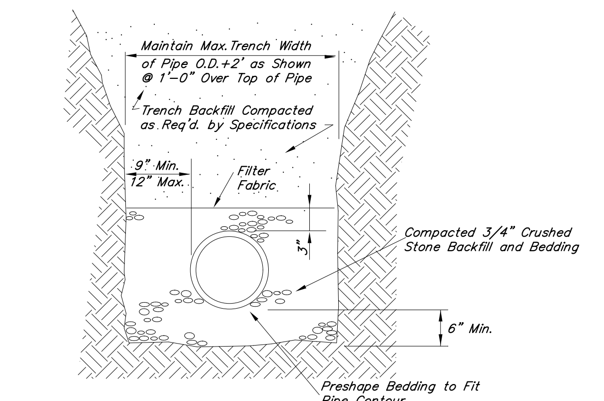
SANITARY SEWER BEDDING DETAIL
