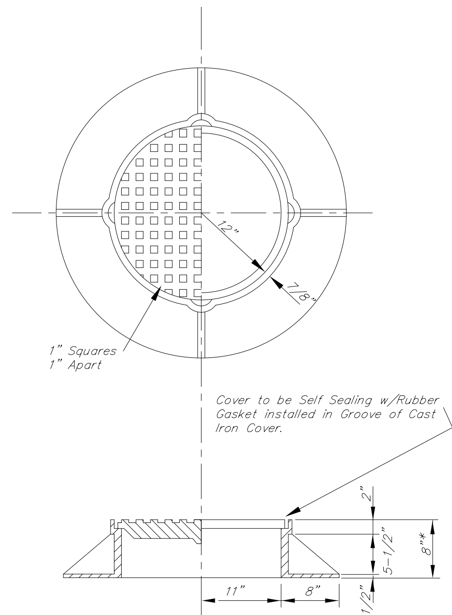
* 4" FRAME ALLOWED WHERE REQUIRED PLAN AND SECTION CAST IRON MANHOLE FRAME & COVER SCALE: 1"=1'-0"
